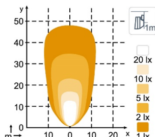
Pictor 620, 1800lm Flood TD US
