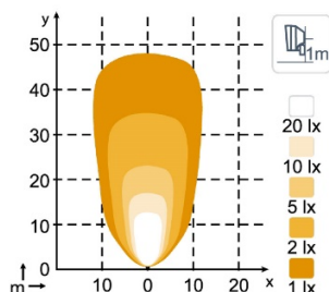
Pictor 620, 1800lm Flood TT DS
