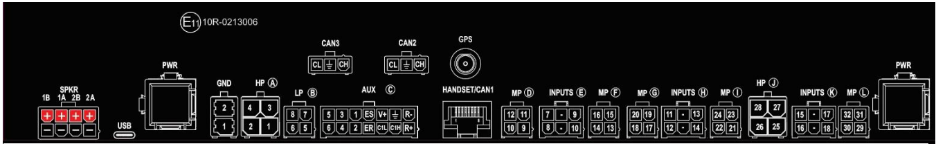
Figure 1 Connector Layout
